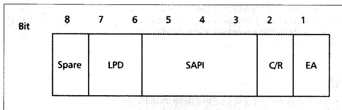
■ Figure 4. LAPDm "address field" format.
