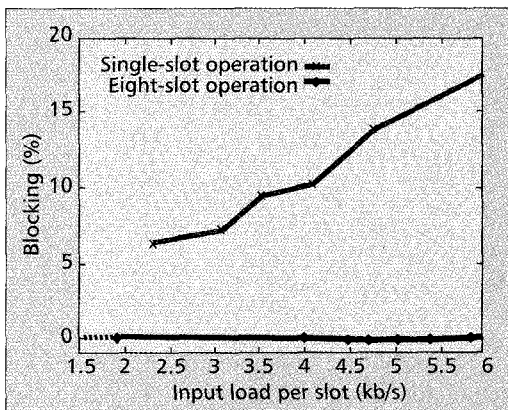
■ Figure 15. Multislot vs. single-slot operation: blocking comparison.
