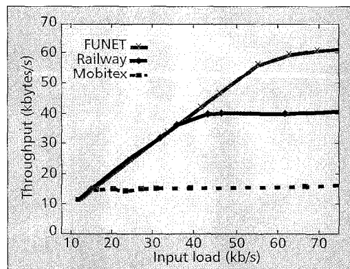
■ Figure 19. Traffic model effects: throughput comparison.
