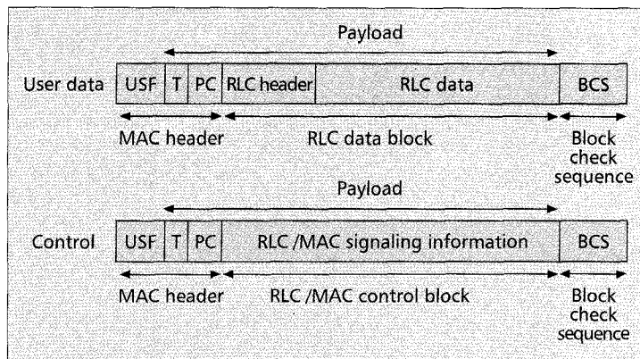
■ Figure 6. GPRS radio block structure.
