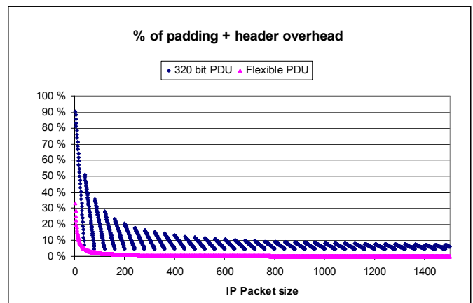
Figure 3. The sum of the padding and header overhead relative to the IP packet size for fixed and flexible RLC PDU sizes.
