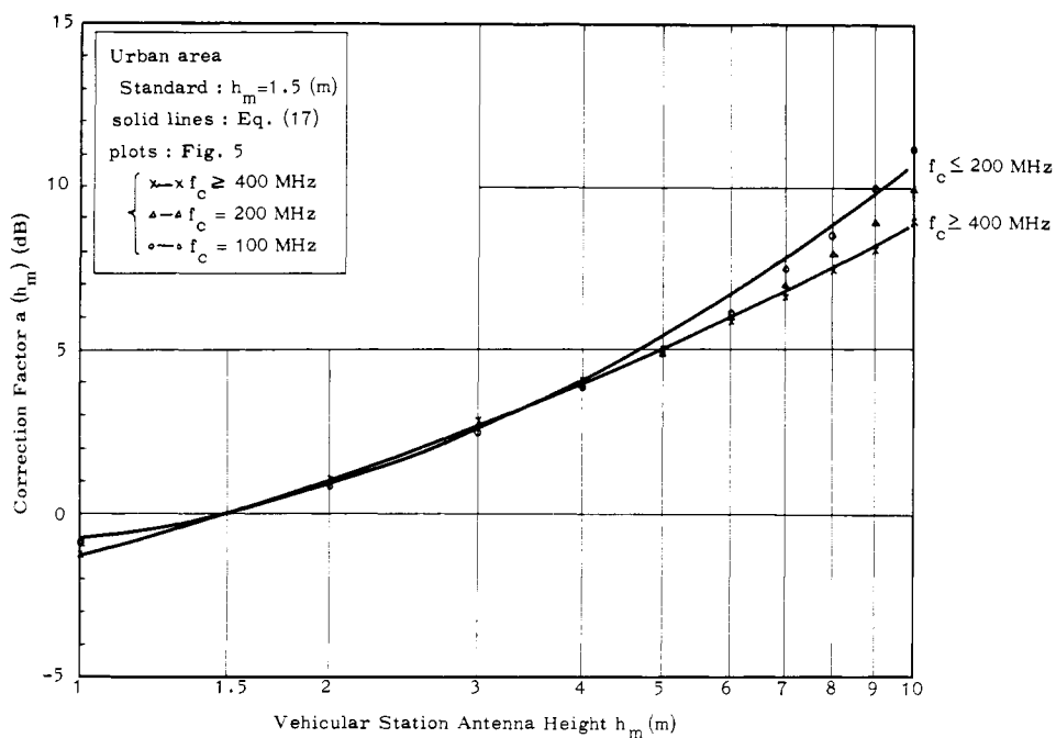
Fig. 8. Correction factors in a large city (2).
