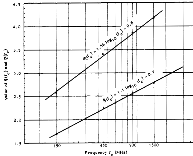
Fig. 6. Determination of coefficients \xi(f_c) and \eta(f_c) .
