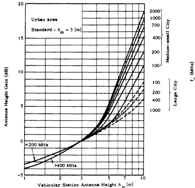
Fig. 4. Prediction curves for vehicular antenna height gain in an urban area.
