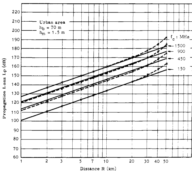
Fig. 9. Propagation loss in an urban area (1).
