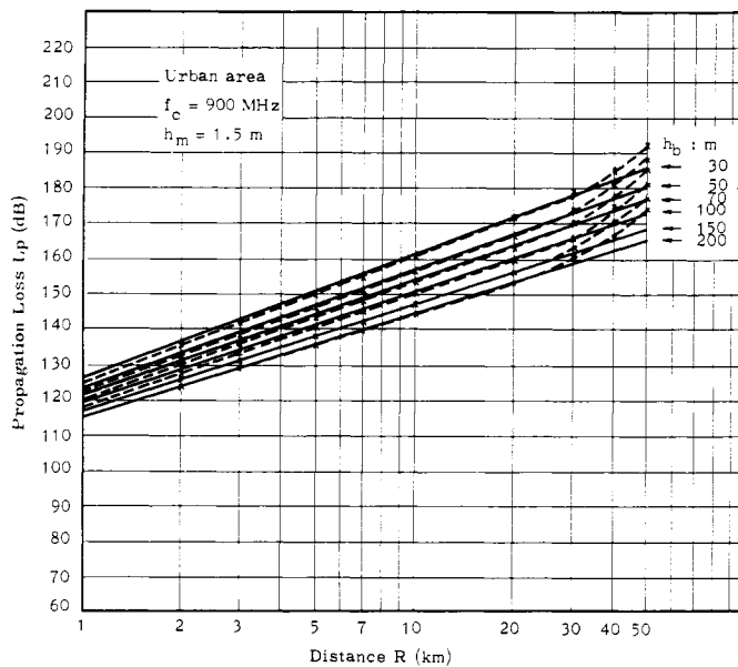
Fig. 10. Propagation loss in an urban area (2).
