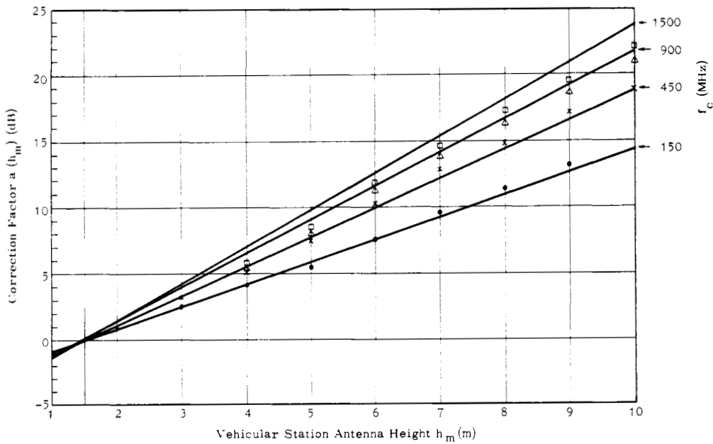
Fig. 11. Correction factors in a medium-small city (2).
