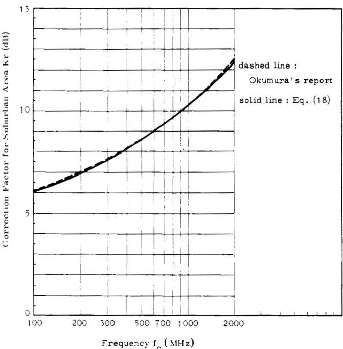
Fig. 12. Correction factor for suburban area.
