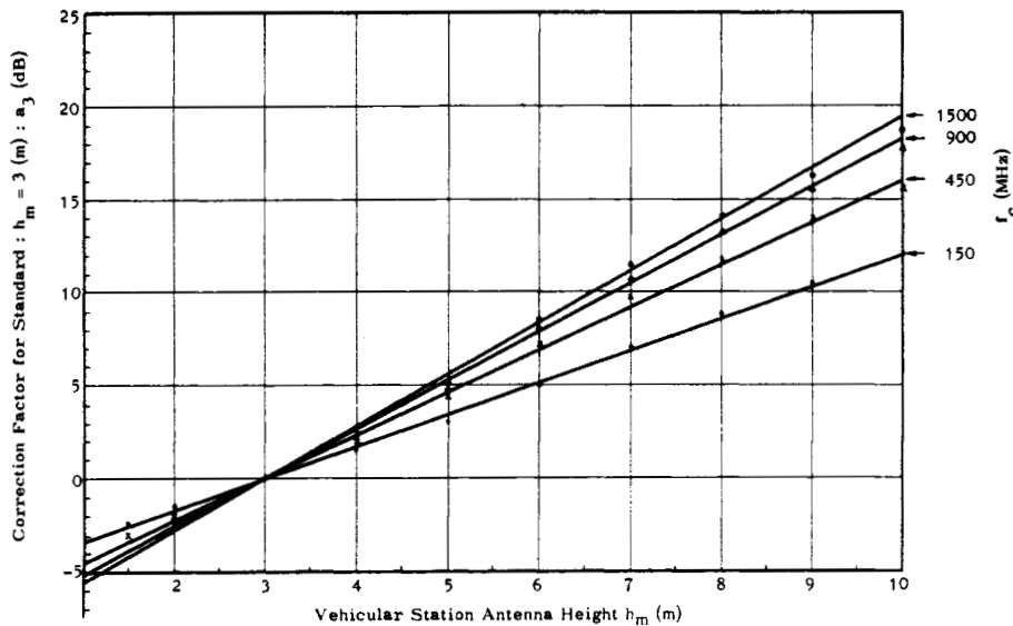
Fig. 5. Correction factors in a medium-small city (1).
