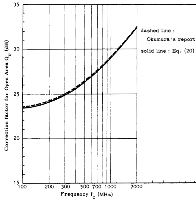
Fig. 13. Correction factor for open area.
